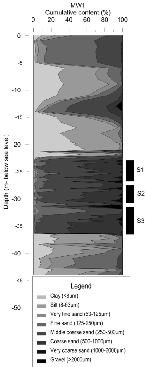
Figure 6: Cumulative grain size contents observed at MW1 (at 5 m from ASR well 1). S1-S3 mark the depth intervals of the ASR well screens.
