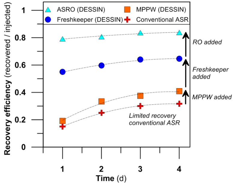
Figure 15: Most relevant results of the SEAWAT modelling study: an increase in recovery efficiencies at the Westland target aquifer thanks to the introduction of the MPPW, the Freshkeeper, and ASRO.
