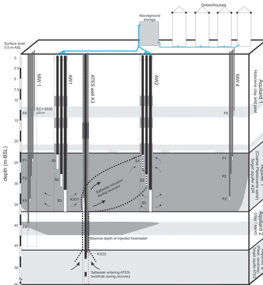
Figure 13: Deep saltwater intrusion via a borehole during recovery of injected freshwater at the Westland ASR site.
