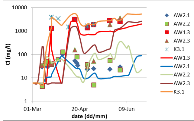
Figure 12: Modelled and observed Cl-concentrations at the most relevant well screens.
